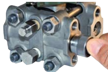
1/4" IEC Transmitter Ports Compatible to 1/4" (IEC 61518) 2.126 (54) process flange ports
