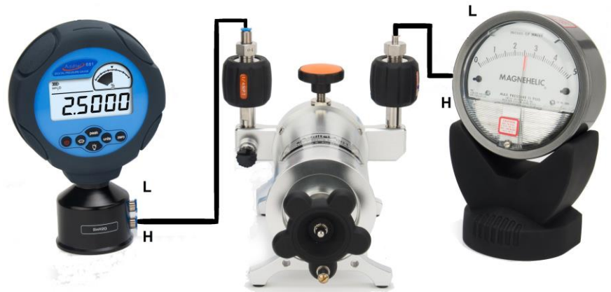
Figure 2 ADT681 DP gauge and ADT901 pump
